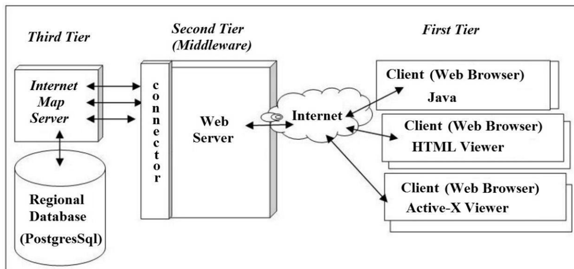
Fig. 2. System Architecture of a web-based Geoportal application [10]
